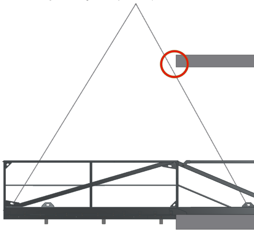
Drawing 5. Sling assembly for transport.
