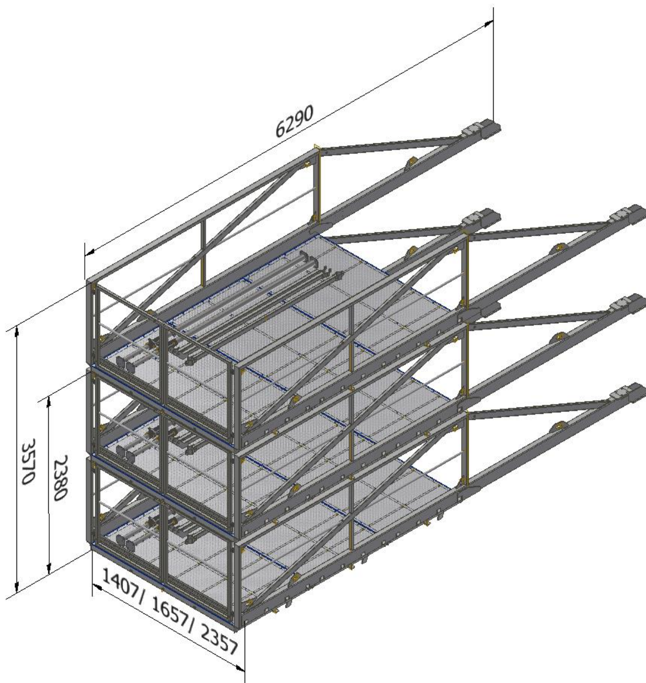
Drawing 10. Transport and storage of assembled platform
