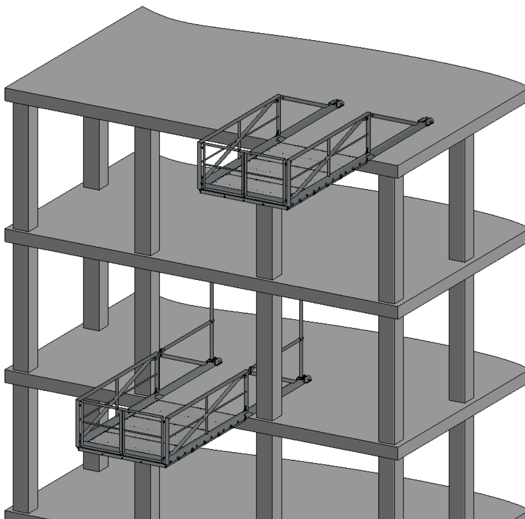
Drawing 1. Unloading platforms
