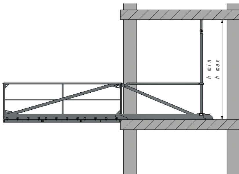
Drawing 2. Assembly between ceilings.
