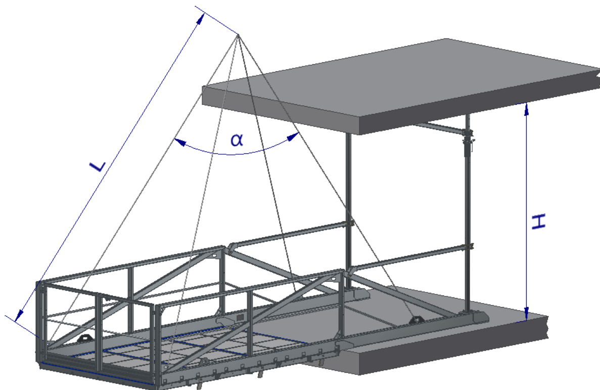
Drawing 5. Sling assembly for transport.
