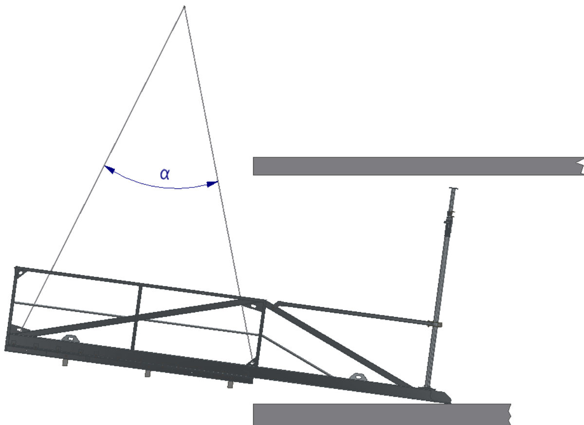
Drawing 7. Transport of tilted platform to installation place.
