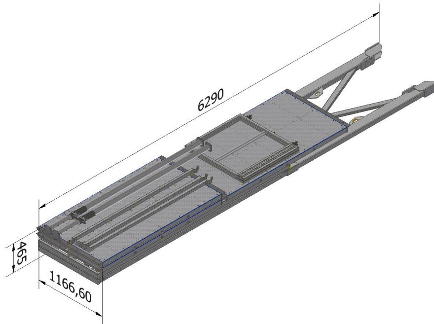
Drawing 8. Transport and storage of unloading platform
