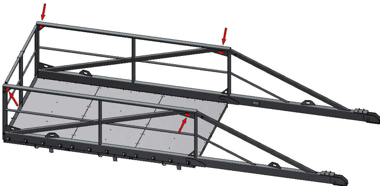
Drawing 4. Safety harnesses attaching points
