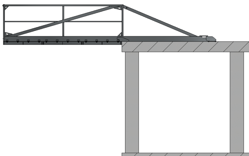
Drawing 3. Assembly by anchoring to the roof.
