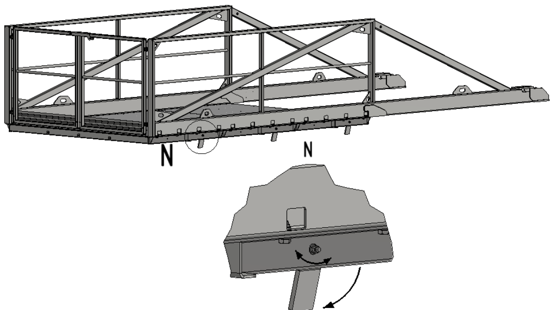
Drawing 9. Unfolding platform feet.
